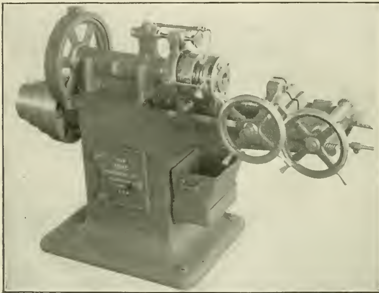
TANDEM DIES ON ACME BOLT CUTTER.
